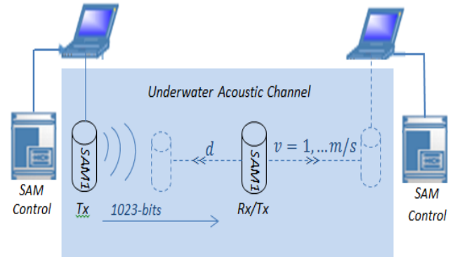
Figure 7: Underwater Mobile Acoustic Sensor Network
