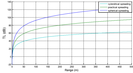
Figure 4: Overall transmission loss ( f = 50\text{KHz} ).
