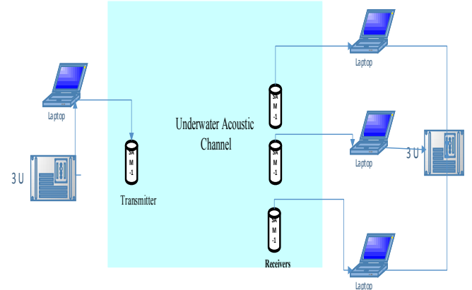
Figure 2: Parallel underwater wireless sensor network
