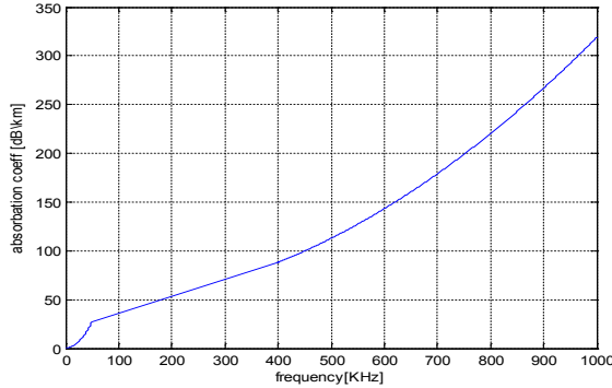
Figure 3: Absorption Coefficient
