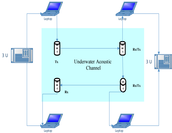
Figure 1: Cascaded underwater wireless sensor network
